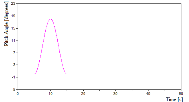
Fig.10: Pitch control behavior
