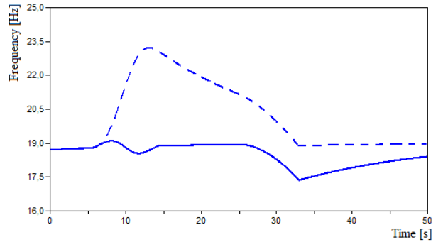
Fig. 9: PMSG terminal voltage frequency behavior
