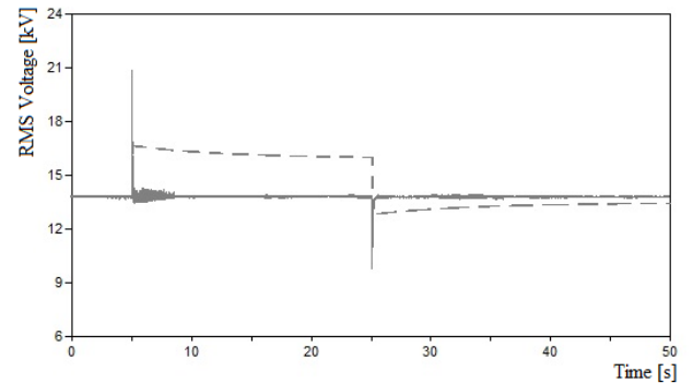
Fig. 14: Isolated load voltage behavior
