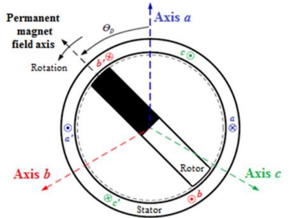
Fig. 3. PMSG physical topology
