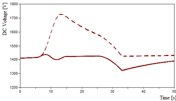
Fig. 11: DC link voltage behavior
