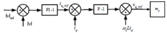
Fig. 6: Block diagram of load voltage magnitude control
