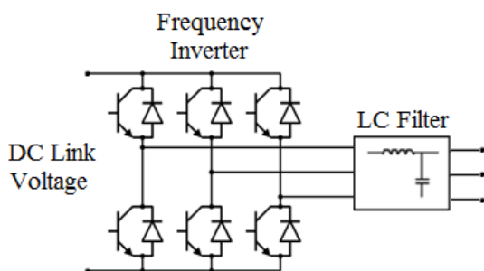
Fig. 5: Frequency inverter topology
