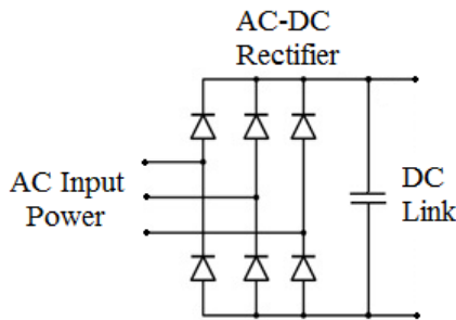
Fig. 4: Full-wave rectifier and the DC link topology
