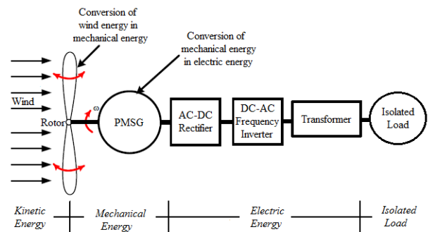
Fig. 1. Electromechanical topology of WECS
