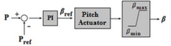
Fig. 2. Pitch angle control block diagram
